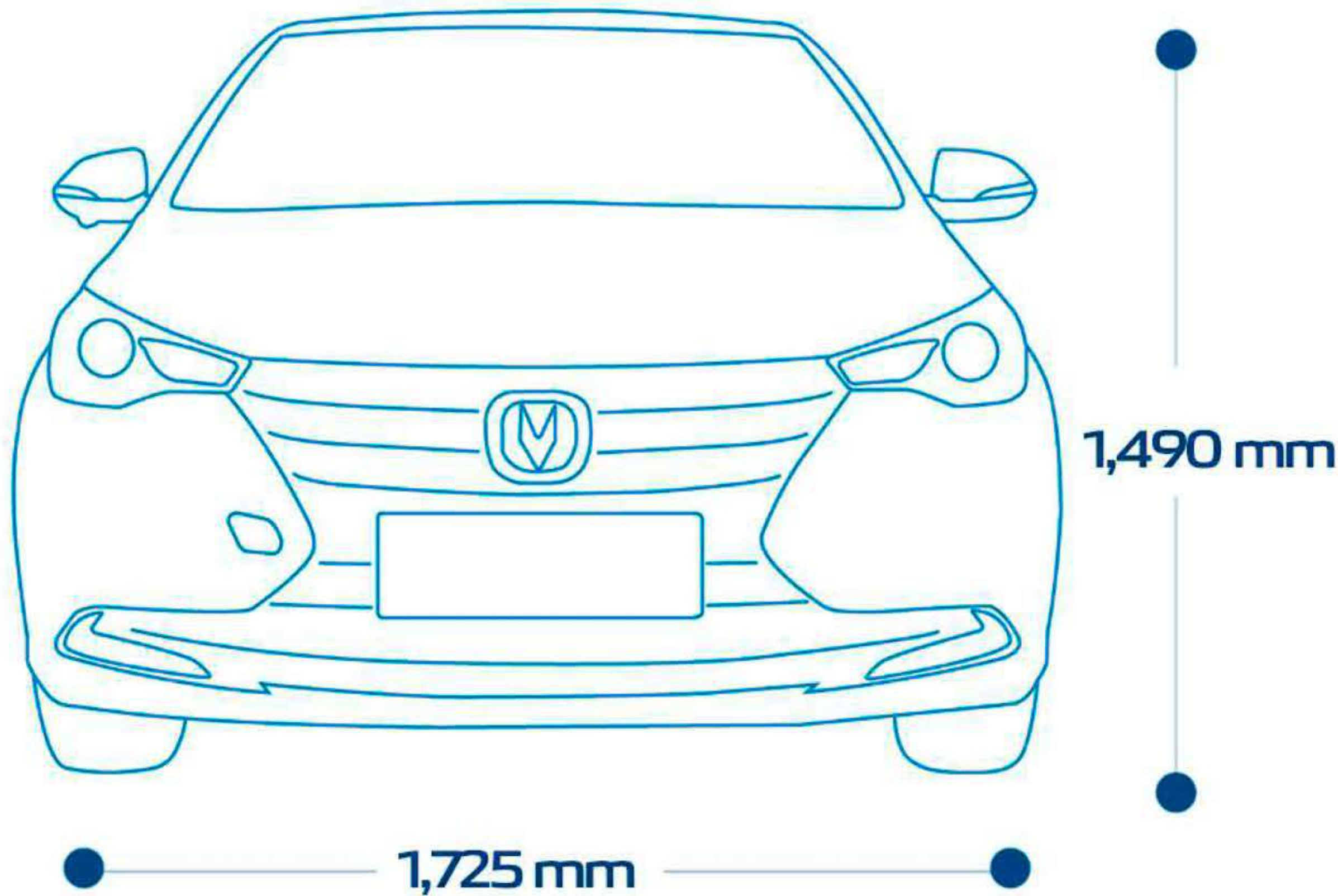
Ancho 1,725 mm
